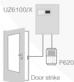
Installation example
